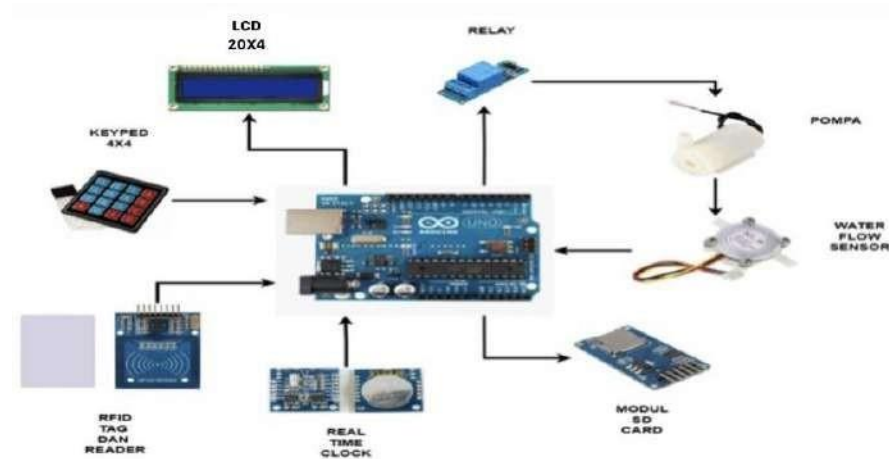
Gambar 2. Diagram Sistem
