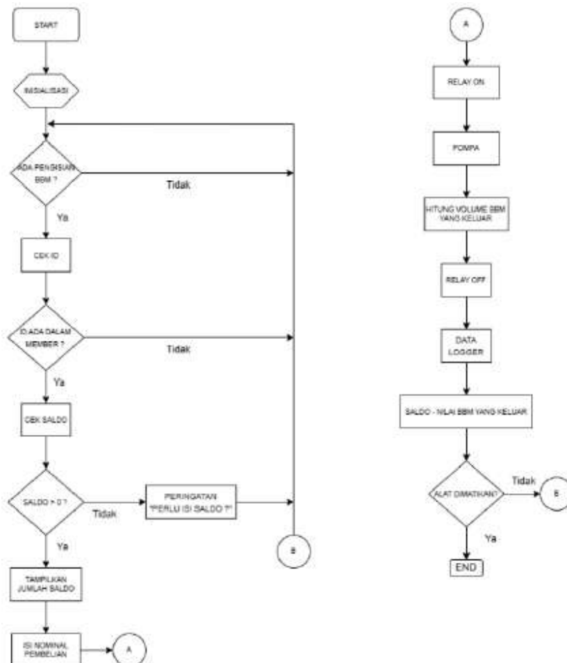
Gambar 3. Flow Chart Perancangan Software
